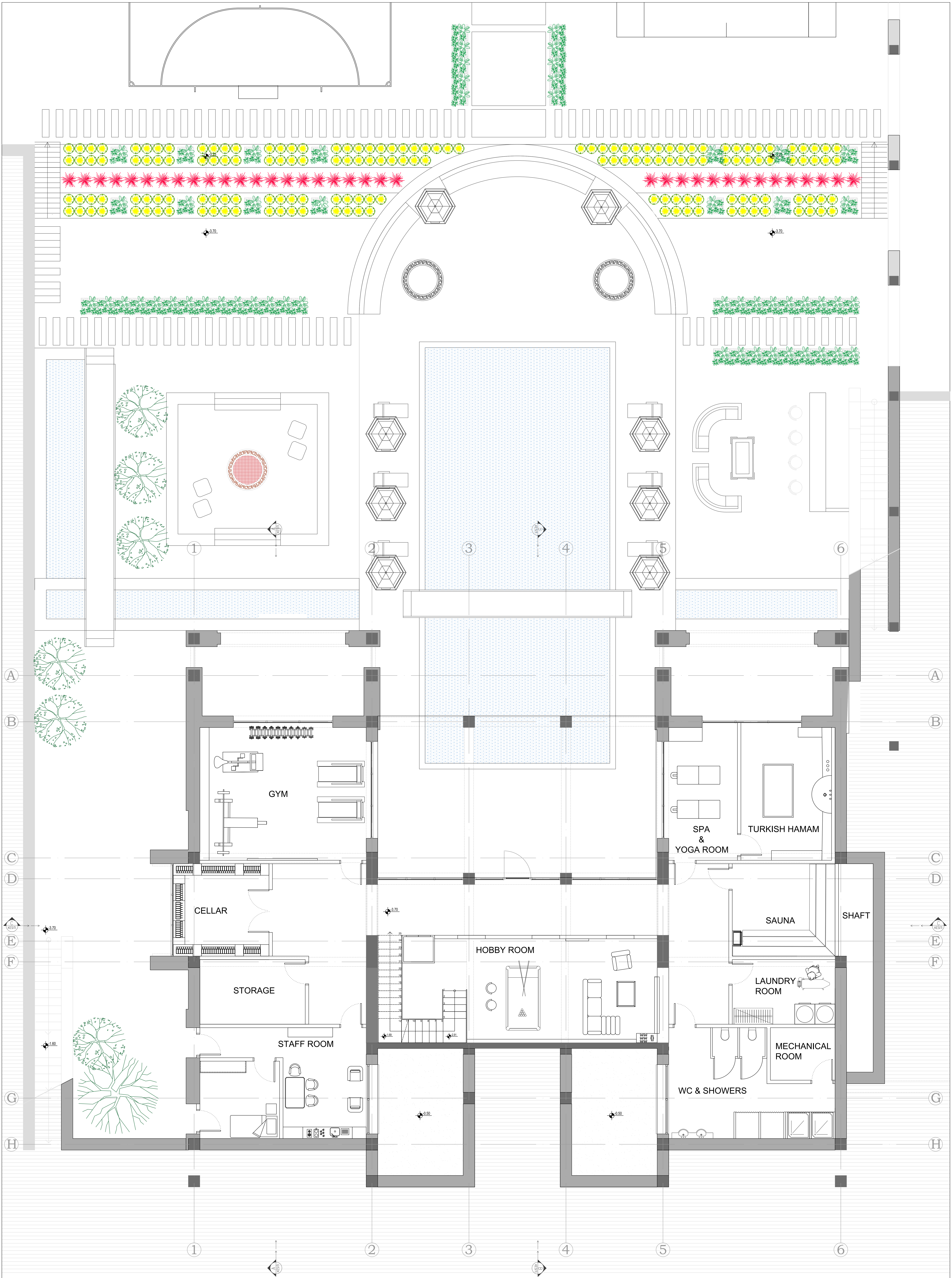
BASEMENT FLOOR PLAN 1:50 SCALE
